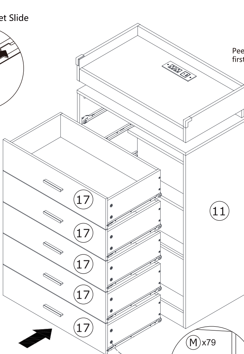
Drawer Slide
